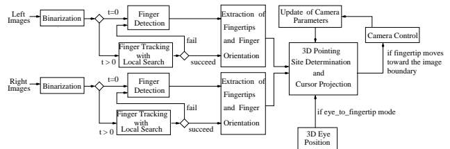
Figure 1. The block diagram of our free-hand pointer.
